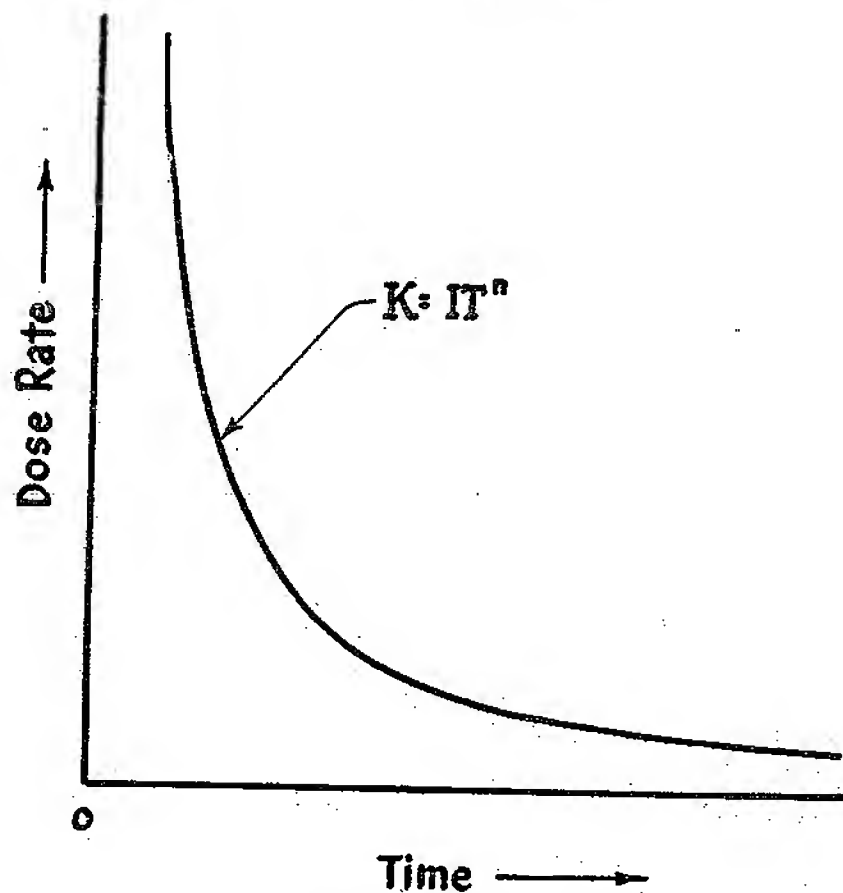
Figure 6—Multiple Decay.
